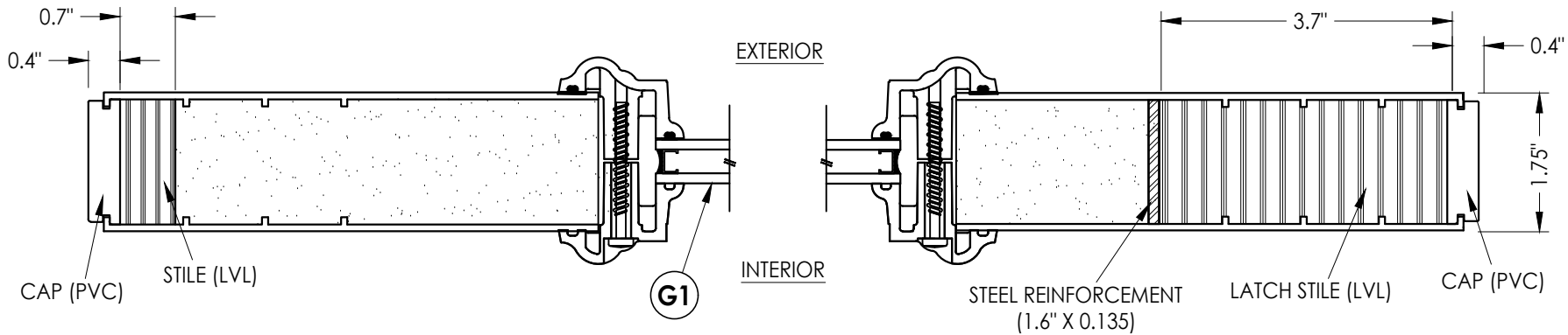
1 4 HORIZONTAL CROSS SECTION
