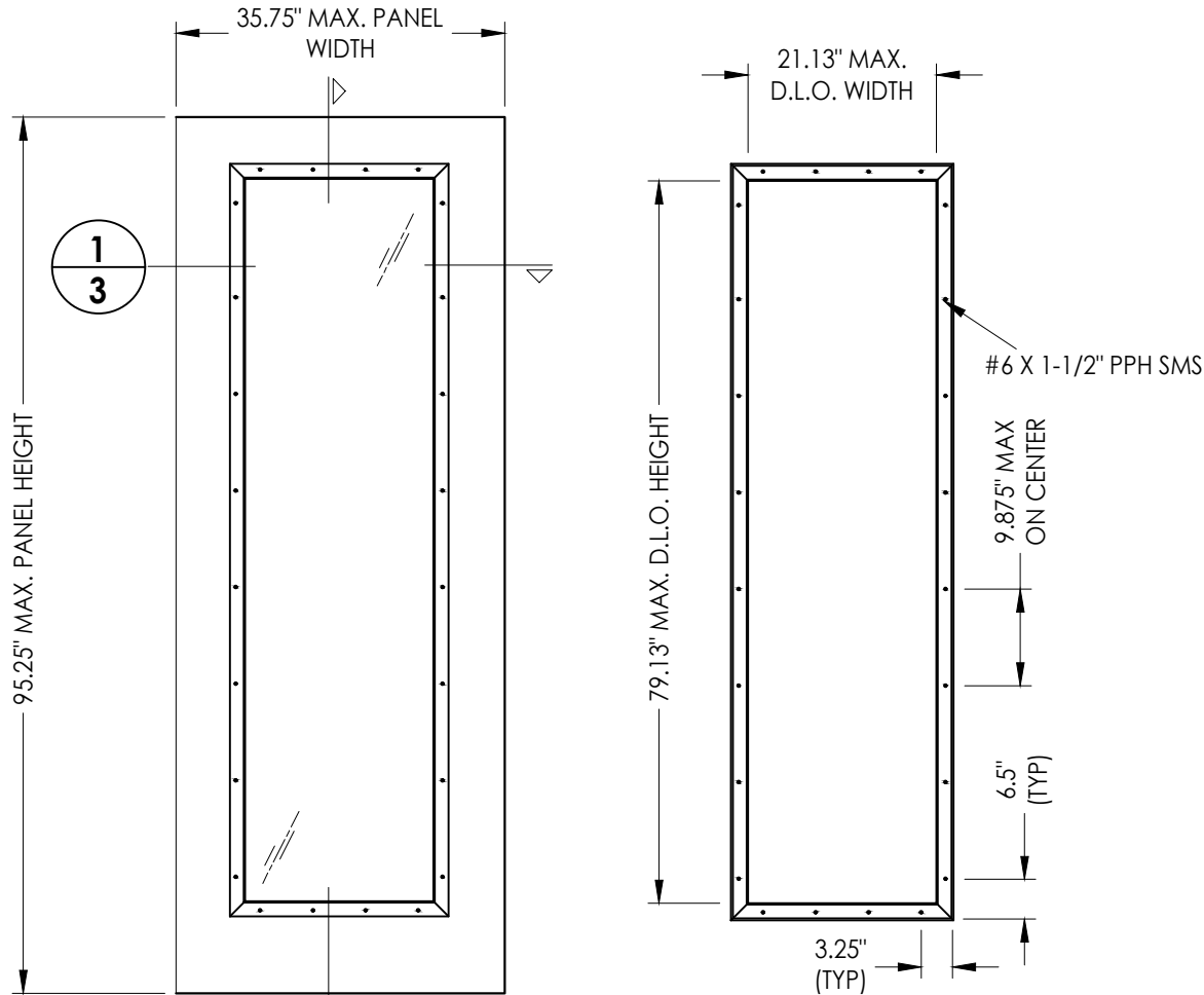
40 2 3 DOOR PANEL Plastpro Fiberglass
